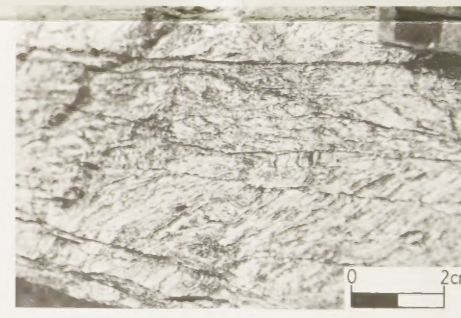
Figure 9. Outcrop photo viewed looking east at Phase Four shear bands. The Phase Four fabric evolves by shearing-out the Phase Three folds, developing into micro-rich, spaced, shear bands (S 4 ). These bands clearly truncate and offset the prevailing mylonitic schistosity (S 2 ). Note the planarity of this fabric. Some shear bands appear discontinuous along strike, and are believed to have only minor displacement across them.
